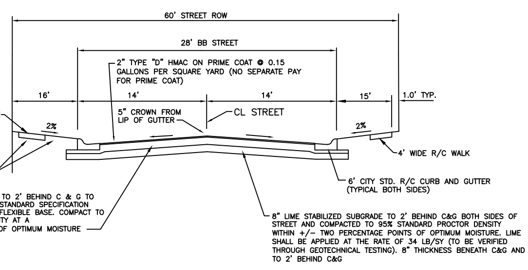
TYPICAL STREET SECTION - 60' ROW NTS
